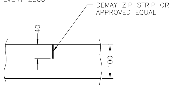
DETAIL A (CONTRACTION JOINT)
